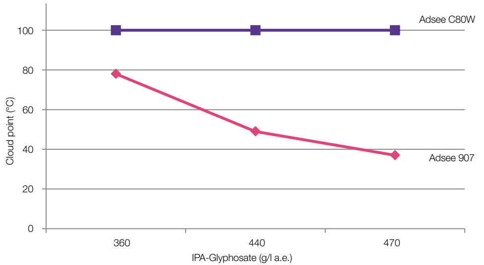
Cloud point of IPA-glyphosate formulations with two different surfactants; Adsee 907, Adsee C80W . Surfactant concentrations are 10 wt-% in all formulations
