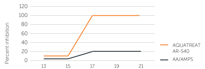
Figure 3: Calcium phosphate inhibition with 15% polymer
