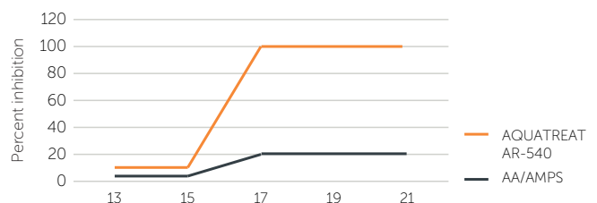
Figure 3: Calcium phosphate inhibition with 15% polymer
